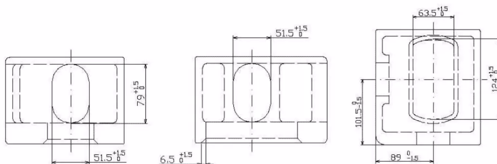
Bottom corner fitting
