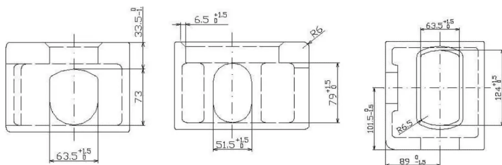
Top corner fitting
