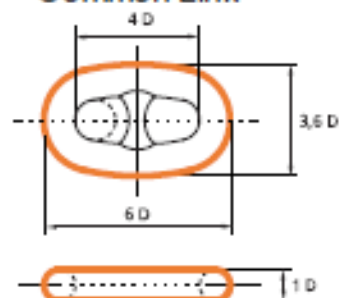
Common Link
